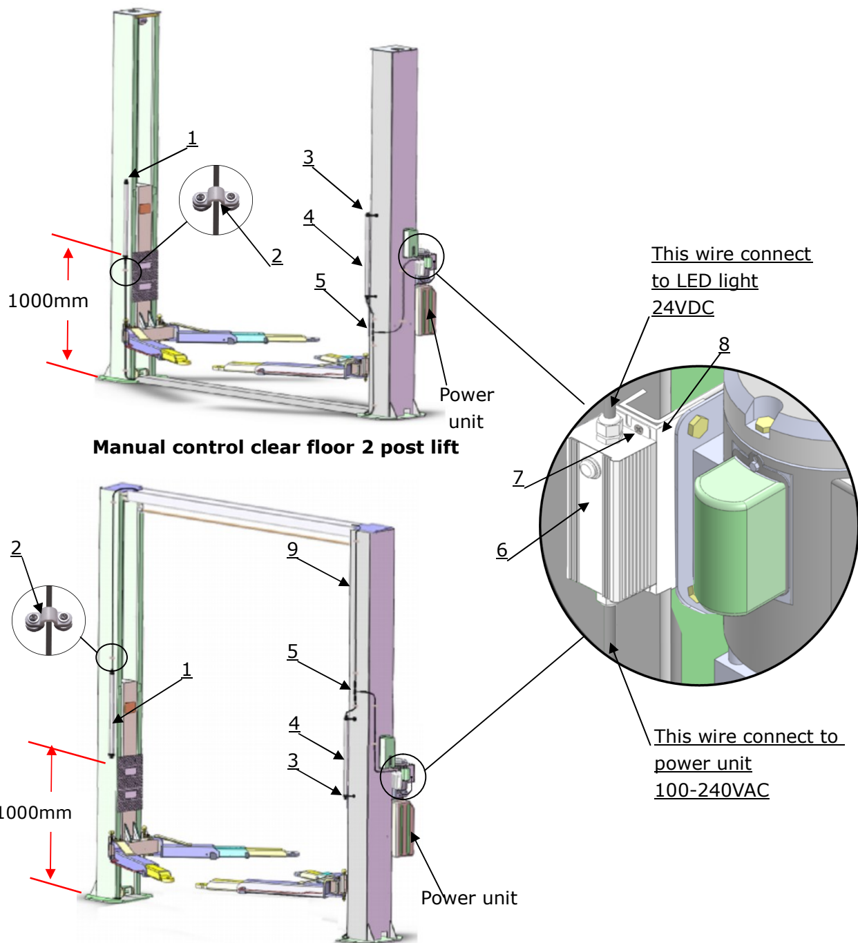
Manual control base-plate 2 post lift
