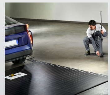
BLIND SPOT RADAR REFLECTOR
