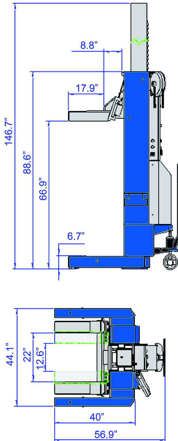
Fig.1 Mobile Column Lift Dimensions
