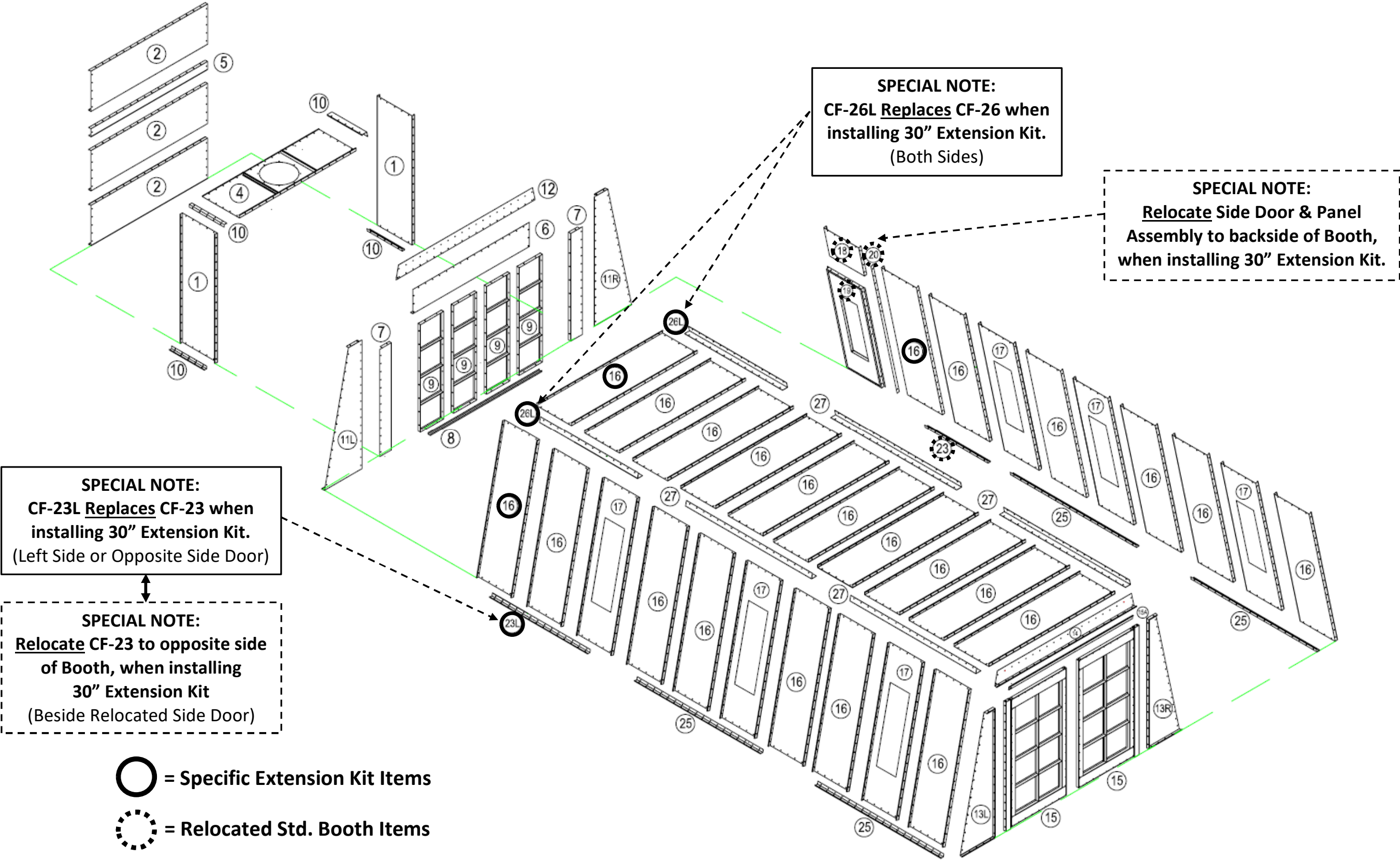
PSB-AFCF23-AK with (PSB-AFCF-30SEPK-AK) AFCF-30" Solid Extension Panel Assembly Kit
