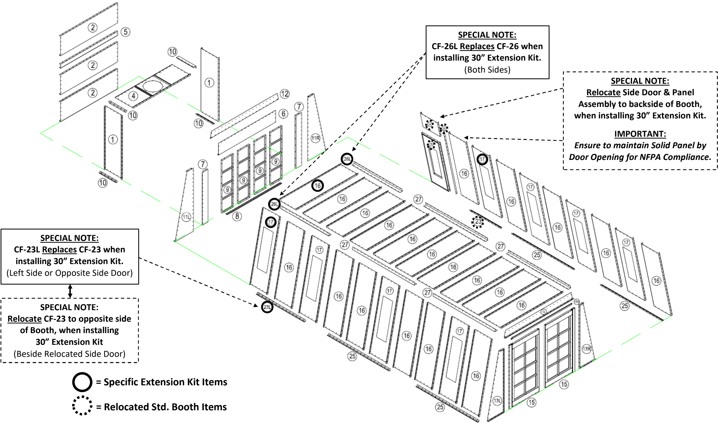
PSB-AFCF23-AK with (PSB-AFCF-30LEPK-AK) PSBAFCF-30" Light Extension Panel Assy. Kit
