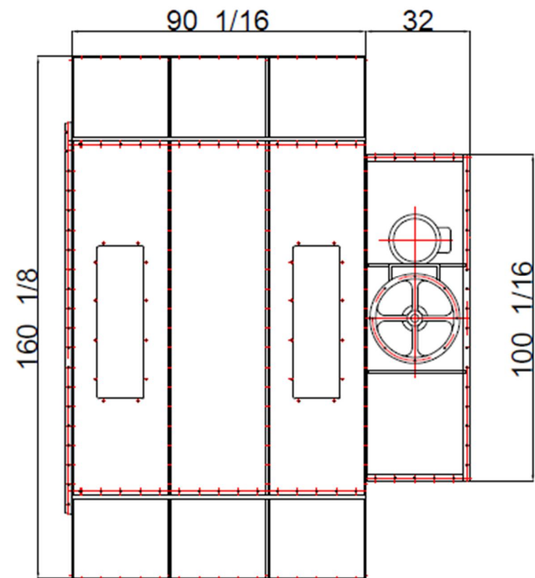
PLAN VIEW
